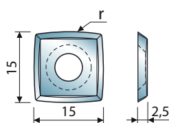
COLTELLO R50 Knife R50
